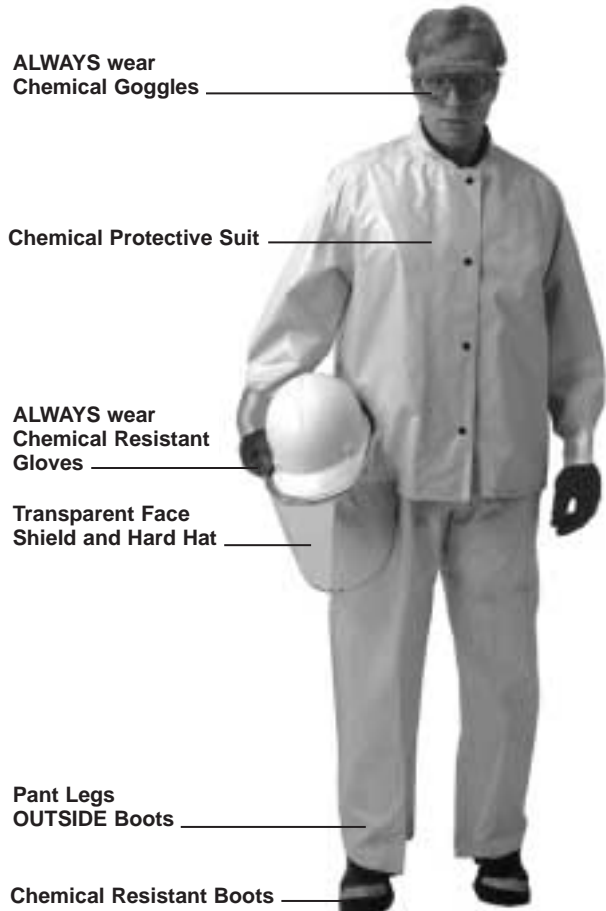
Figure 1 Protective Clothing and Equipment for Handling of Bulk Caustic Soda Solution.
